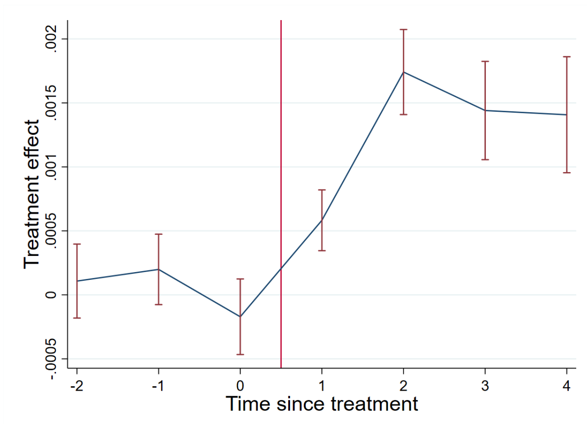
Figure A9: Effect of job loss on crime, two-way fixed effects panel estimates with correction from de Chaisemartin and D'Haultfoeuille (2019)
