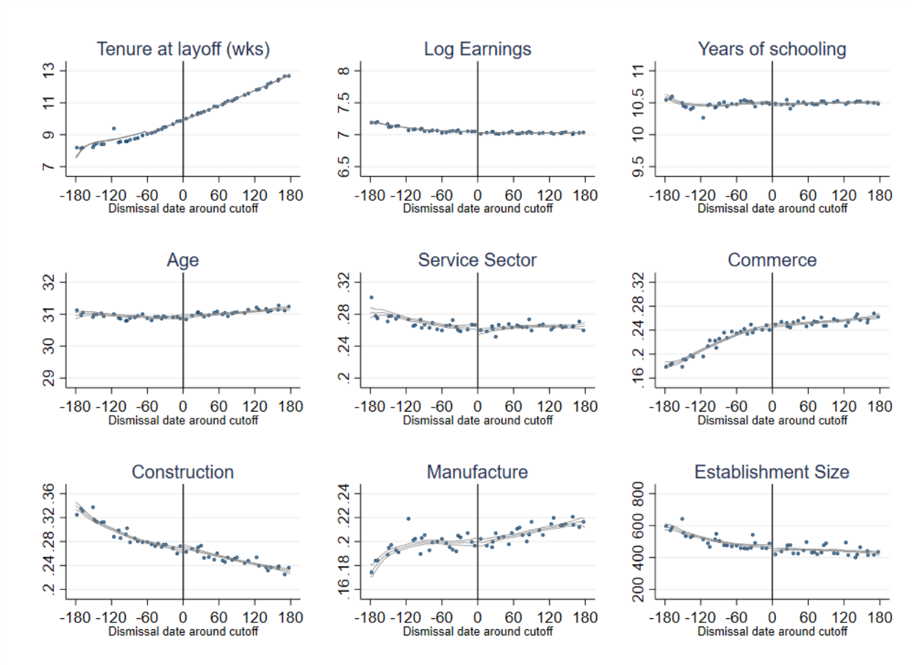
Figure A13: Balance of pre-determined covariates across workers near the cutoff for UI eligibility
