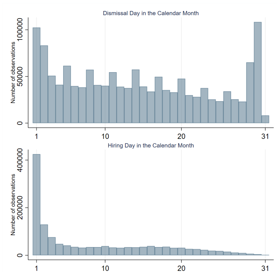
Figure A11: Cyclicalty in hiring and firing of workers
